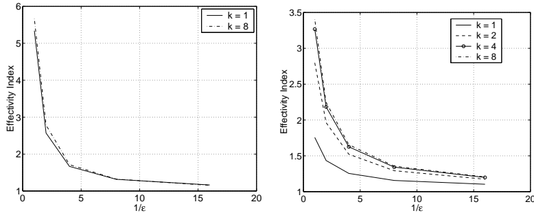
(a) Effectivity Index for H^1 semi-norm estimate using an initial guess of u_0 = 0 . The graphs for k = 2, 4 are similar.
