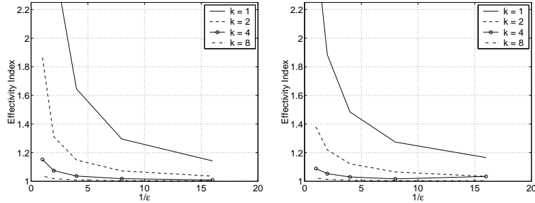
(a) Effectivity Index for H^1 semi-norm estimate with u_0 = 0 .
